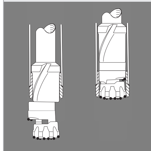
Eccentric under-reamer system
