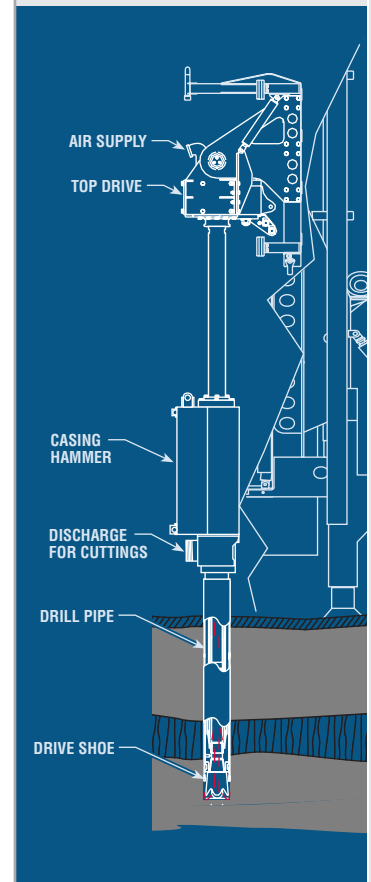
Overview of casing driver system
